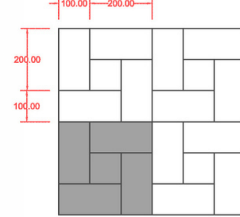
Windmill
