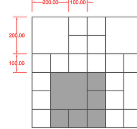
Stepping Stone
