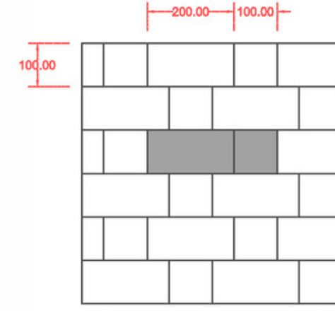
Alternating Horizontal
